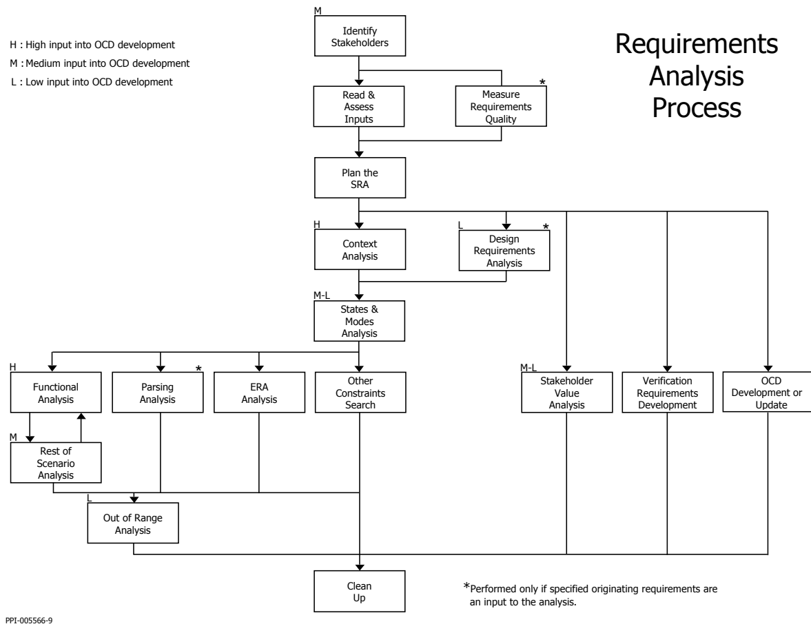
Figure 1: An Effective Requirements Analysis Process
